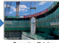
Pressurizer Hoisting July 6, 2023
